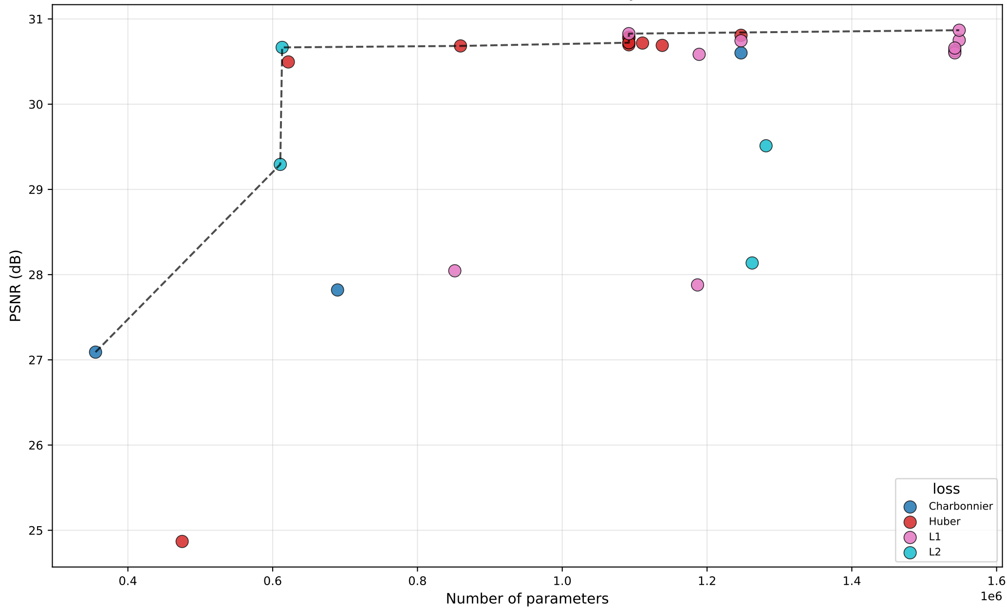
PSNR vs #Params — HAT — by loss
